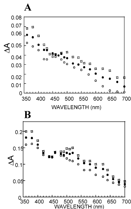
Figure 3. (A) Kinetic difference spectra at 300 ns after pulse radiolysis of dG at pH 2.1 (○), pH 3.8 (●), and pH 6.5 (□). Samples contained 1 mM deoxyguanosine, and 10 mM acetate buffer (pH 2.1 and 3.8) or 10 mM phosphate buffer (pH 6.5). (B) Kinetic difference spectra of pulse radiolysis of dG monitored at 70 (○), 120 (●), 250 ns (□) after pulse radiolysis. Experimental conditions were the same as those described in the legend to Figure 1.
